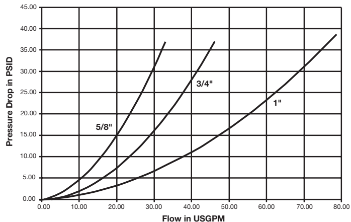
FEM Series (5/8", 3/4" & 1") Test Fluid: Oil - 150 SUS
